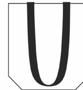
Bag with trapeze bottom with grosgrain tape handles format 470x150x500 mm boxed: 100 pcs palletized: 800
